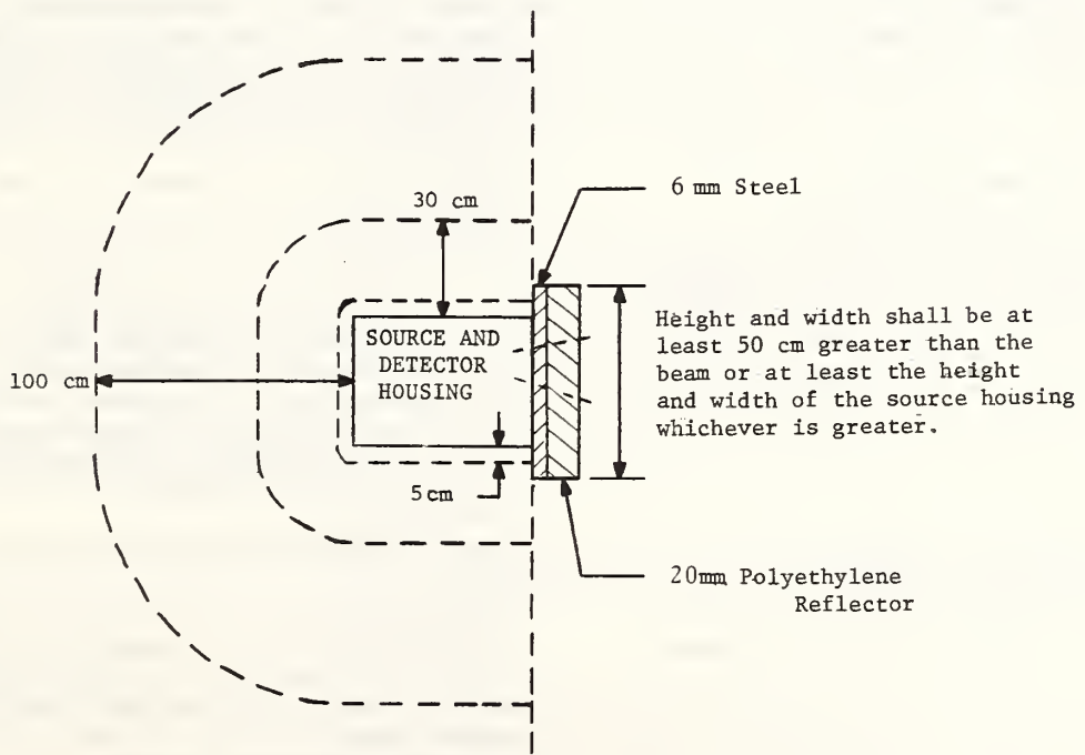
FIGURE IIF. Neutron Backscatter Gauge
